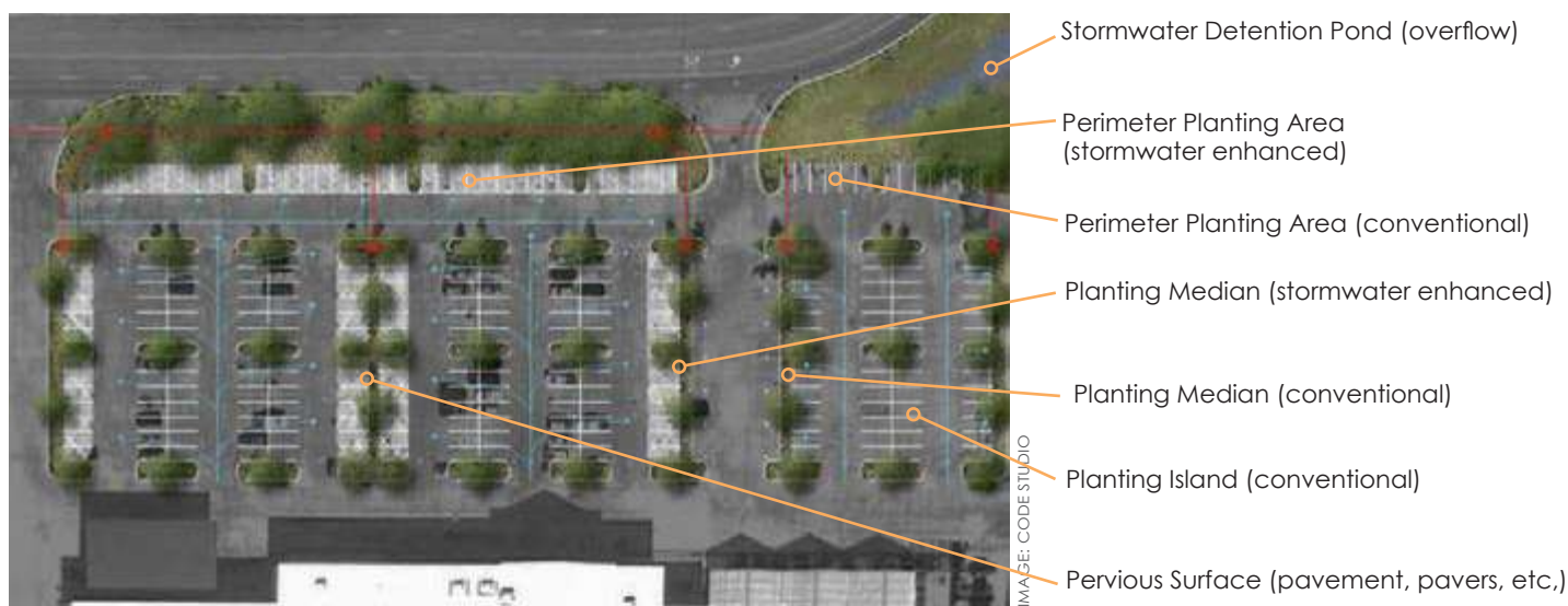
CH7-44: An illustrative example of how the parking lot might be transformed with the application of integrated landscaping and stormwater management approaches. The example above mixes both conventional and stormwater enhanced approaches.
