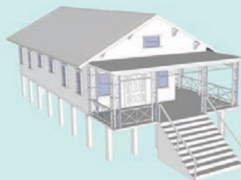
CH5-41: Lift the entire house, with the floor slab attached, and build a new foundation to elevate the house.
