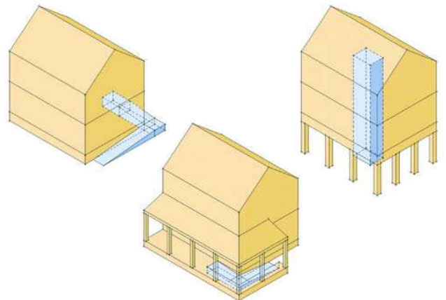
C-3 Accessibility is an important factor in the application of Universal Design principles to residential and commercial buildings. These three techniques provide residential accessibility that complies with FEMA requirements for raising the first floor above the flood plain.
