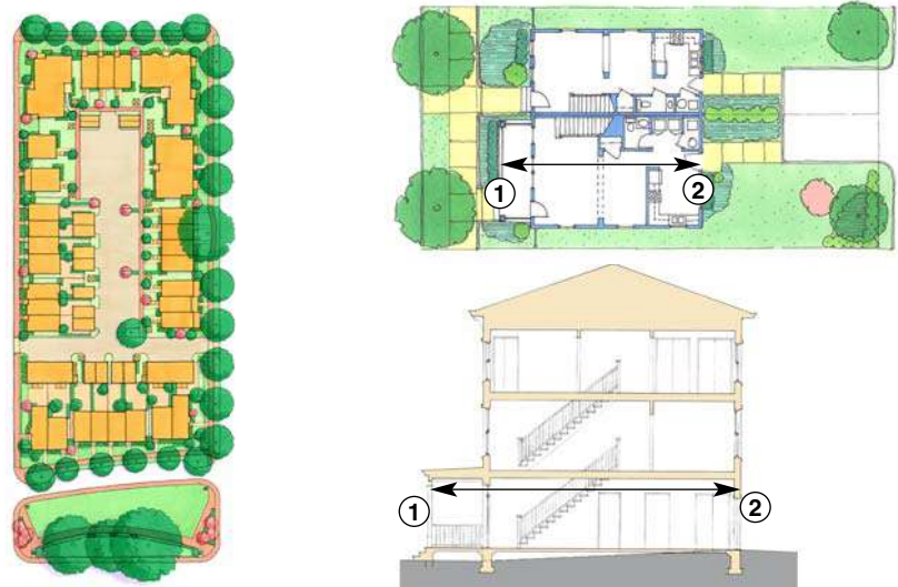
D-58 Left: By raising the elevation of the middle of the block, each building has a zero-step entry from the parking area. Top right: Site detail shows the zero-step entry from the parking area. Bottom right: Cross-section illustrates grading with a raised porch on the street and a zero-step entry from the parking area.
